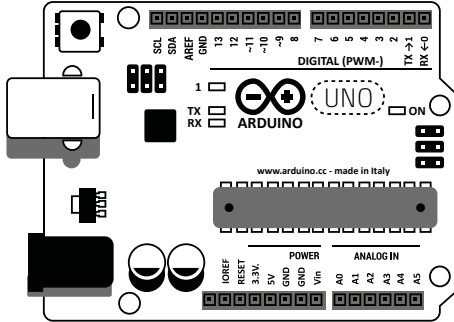
System Arduino
